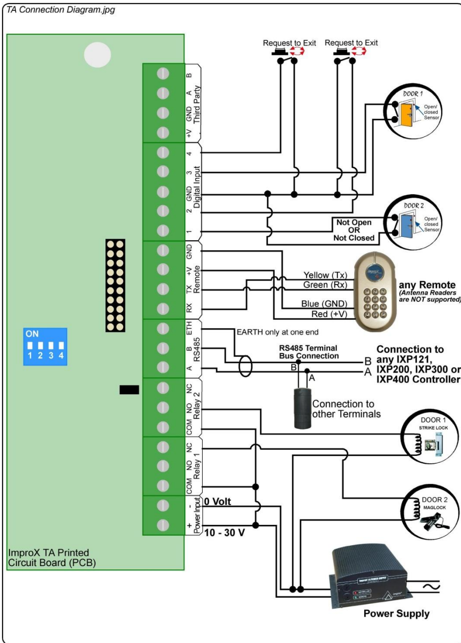
Figure 4: Typical ImproX TA Electrical Connections
