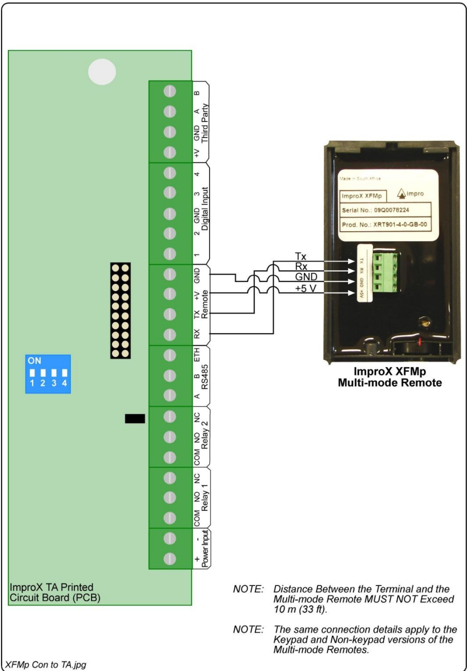
Figure 6: ImproX TA Connected to the Multi-mode Remote Reader
