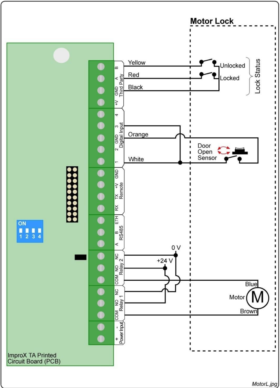
Figure 7: ImproX TA Terminal Connected to the MIWA AL3M Motor Lock
