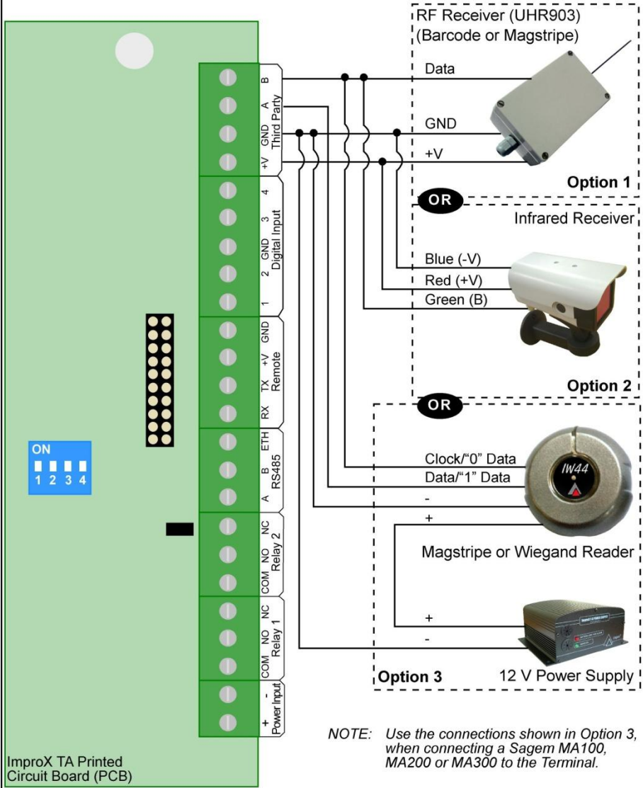
Figure 5: Typical ImproX TA Third-party Port Electrical Connections
