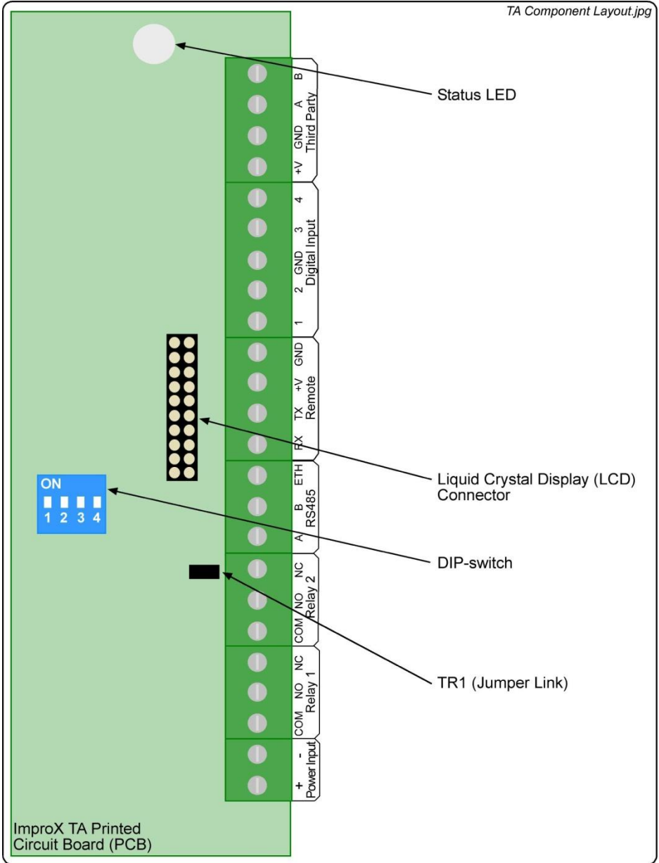
Figure 3: ImproX TA Component Layout Diagram
