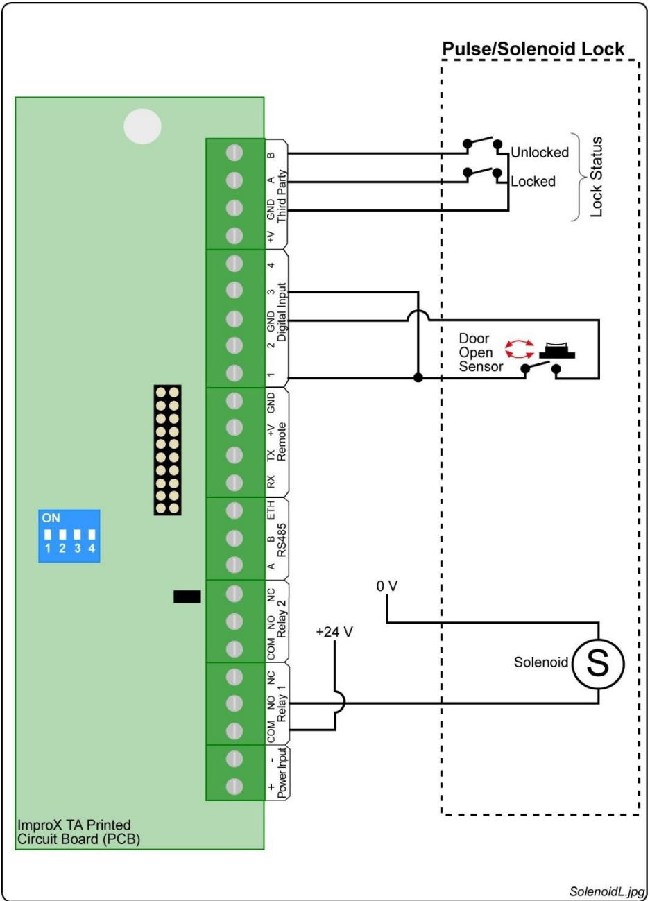
Figure 8: ImproX TA Terminal Connected to a Pulse or Solenoid Lock
