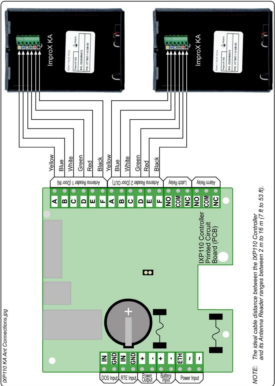
Figure 2: ImproX KA Connected to the IXP110 Controller
