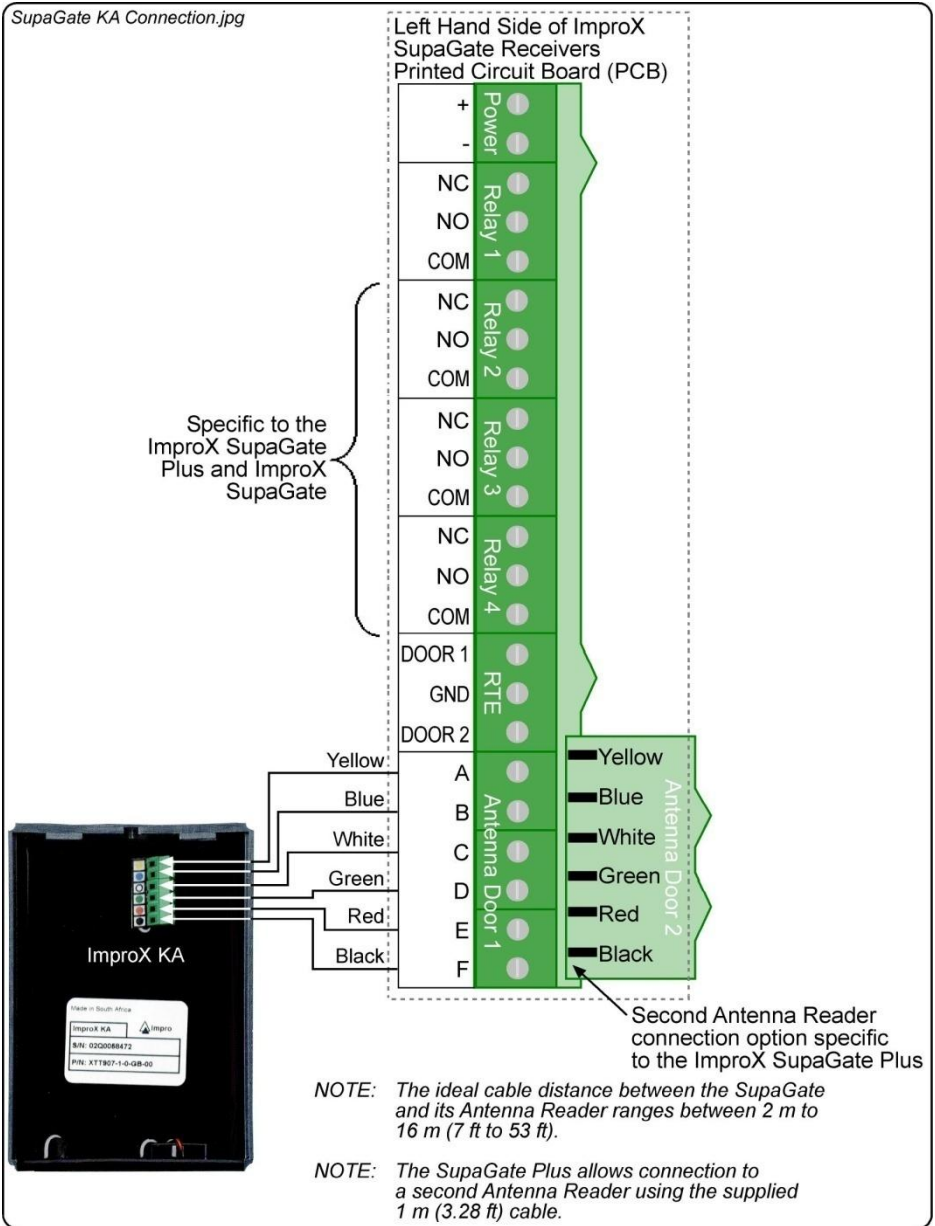
Figure 1: ImproX KA Connected to the SupaGate Receiver
