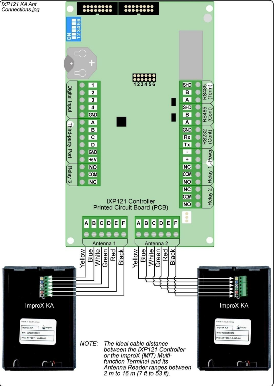
Figure 3: ImproX KA Connected to the IXP121 Controller and ImproX MFT
