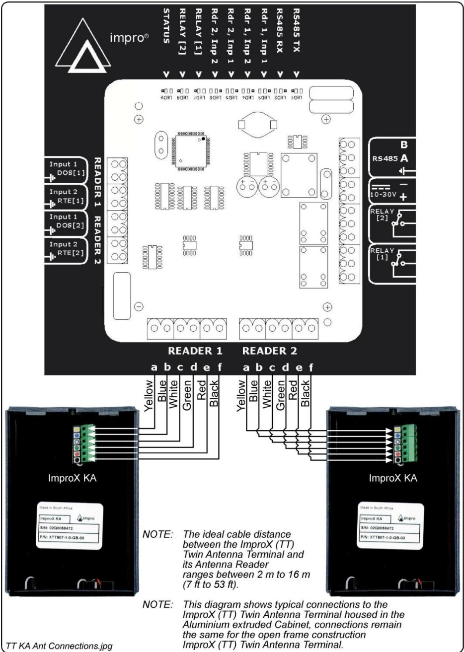
Figure 4: ImproX KA Connected to the ImproX TT
